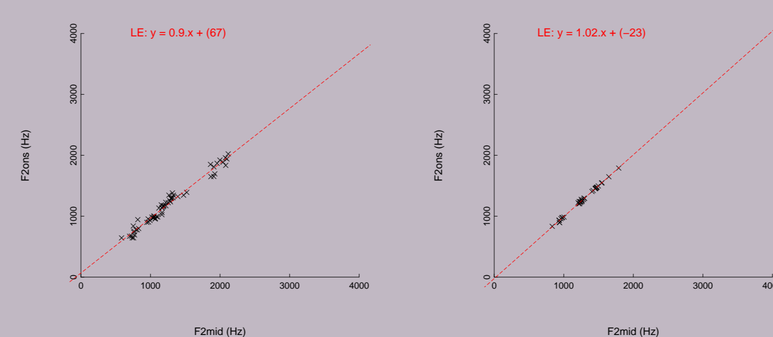
Figure 2: Two locus equation slopes of long (left) vs. short (right) vowels respectively, produced with the consonant /q/ in final position by speaker: L3.
