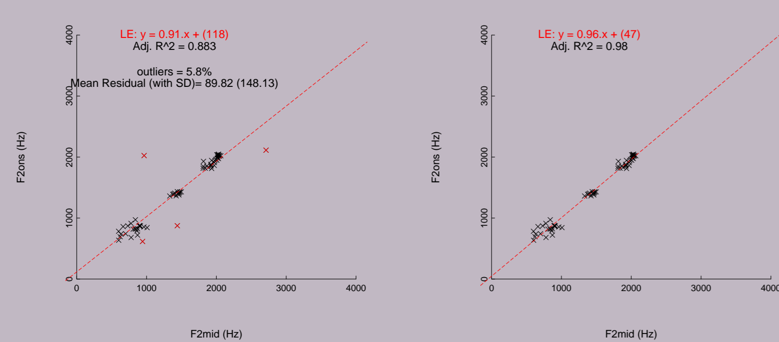
Figure 1: Two representations of a locus equation slope of the consonant /ʔ/ produced by speaker: L1 with long vowels in final position, with and without the outliers respectively.
